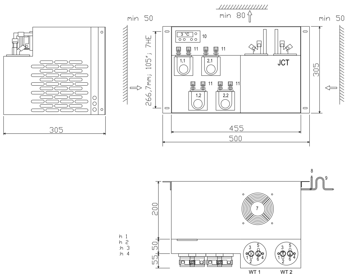
Dimensions Grand Cooler
